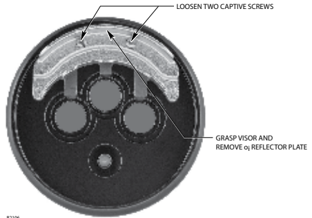
Figure 18— O j Reflector Plate Removal
