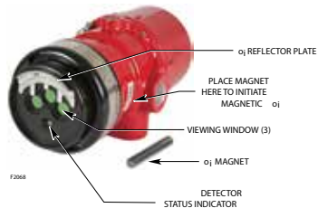
Figure 2—Front View of the X3301
